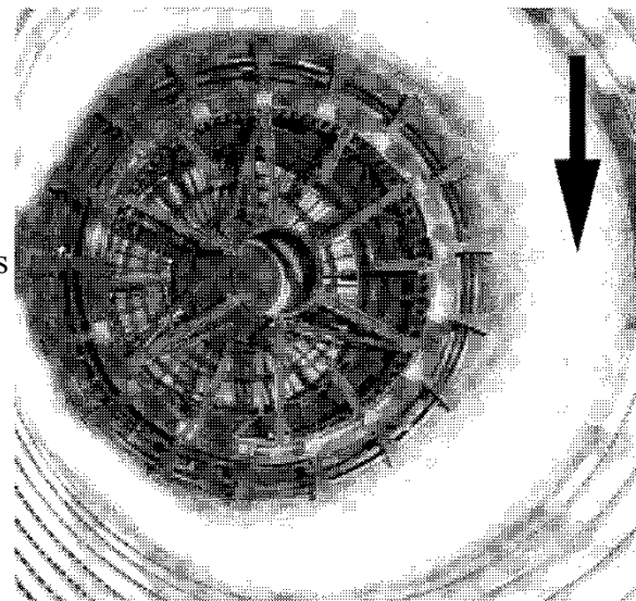
Figure 3.2-30 Screech Liner
