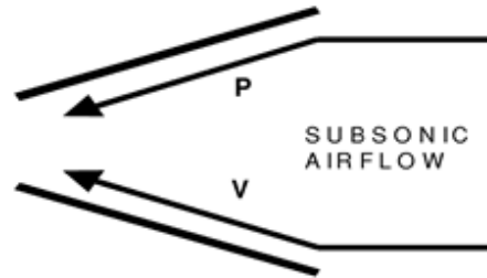
Figure 3.1-1b Subsonic Nozzle
