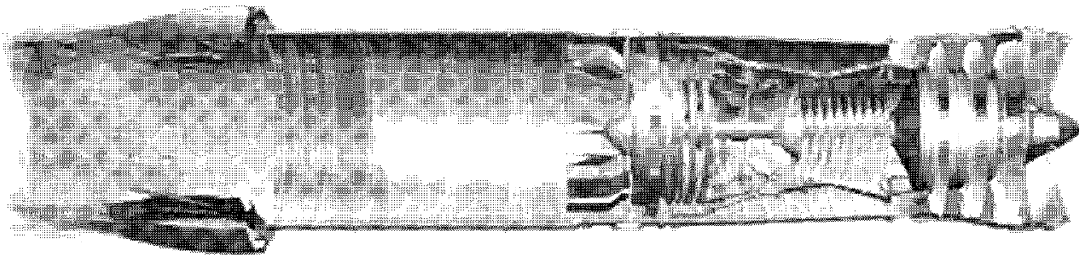
Figure 3.2-26 Gas Generator with Afterburner Unit
