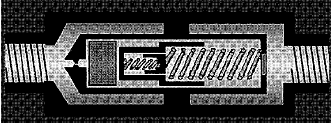
Figure 3.6-10 Hydraulic Fuse
