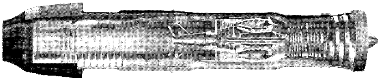
Figure 3.4-6 Turbofan
