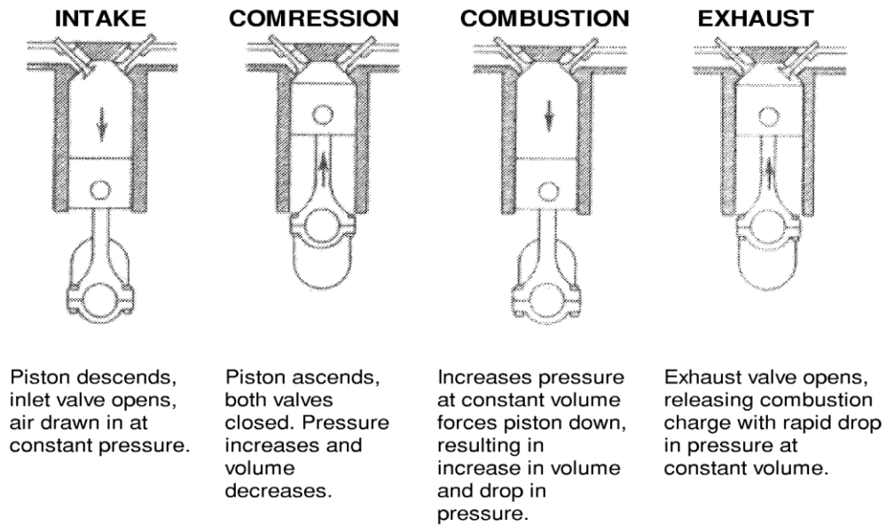
Figure 3.1-5 Otto Cycle
