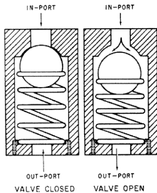
Figure 3.6-7 Check Valve
