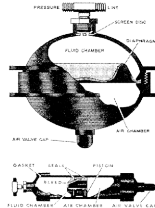
Figure 3.6-8 Accumulators
