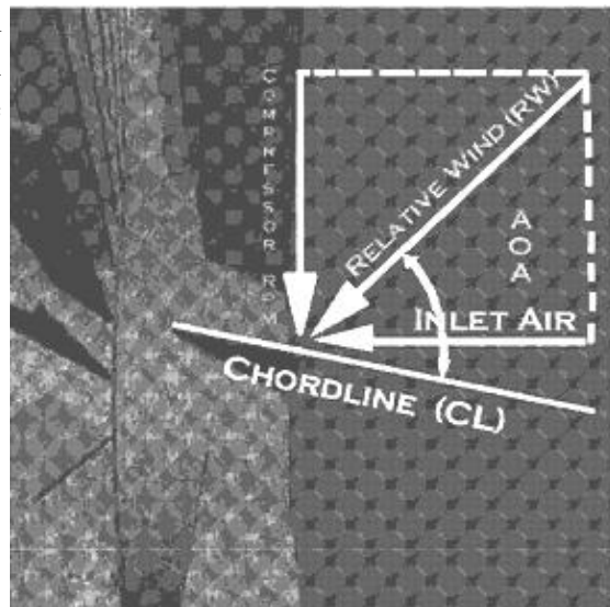
Figure 3.3-1 Angle of Attack
