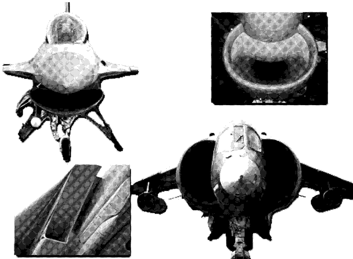
Figure 3.2-2 Inlet Ducts
