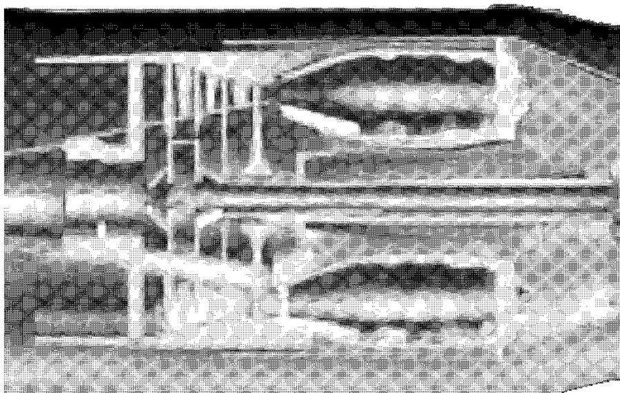
Figure 3.2-15 Burner Section
