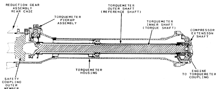
Figure 3.5-5 Torquemeter Assembly
