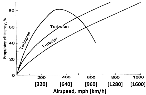
Figure 3.5-8 Thrust Efficiency Graph
