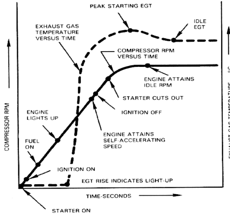
Figure 3.10-4 Starting Cycle
