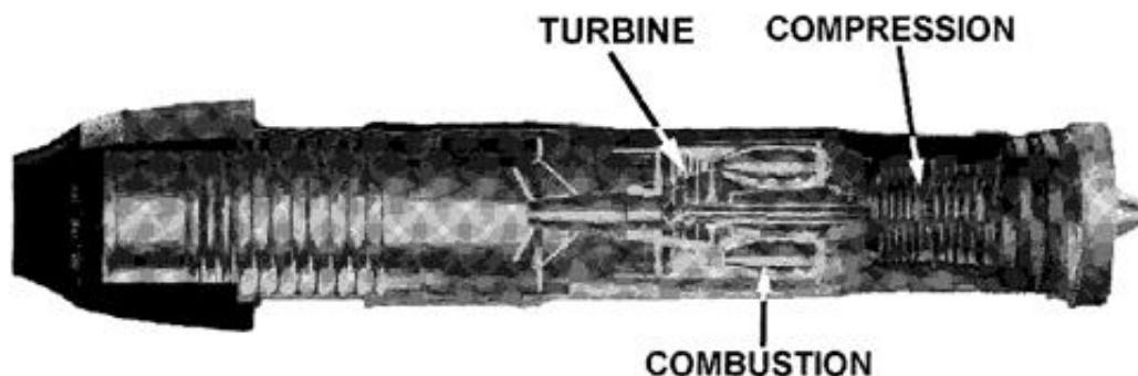
Figure 3.2-1 Gas Generator
