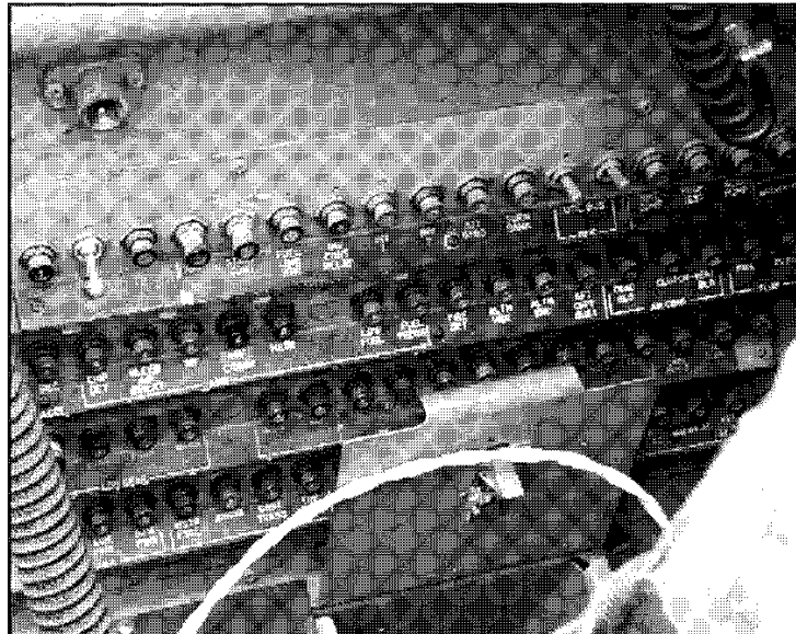
Figure 3.7-6 Circuit Breakers
