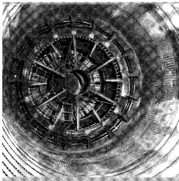
Figure 3.2-27 Afterburner Assembly
