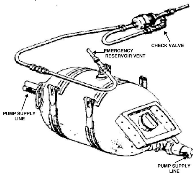
Figure 3.6-4 Nonpressurized Reservoir
