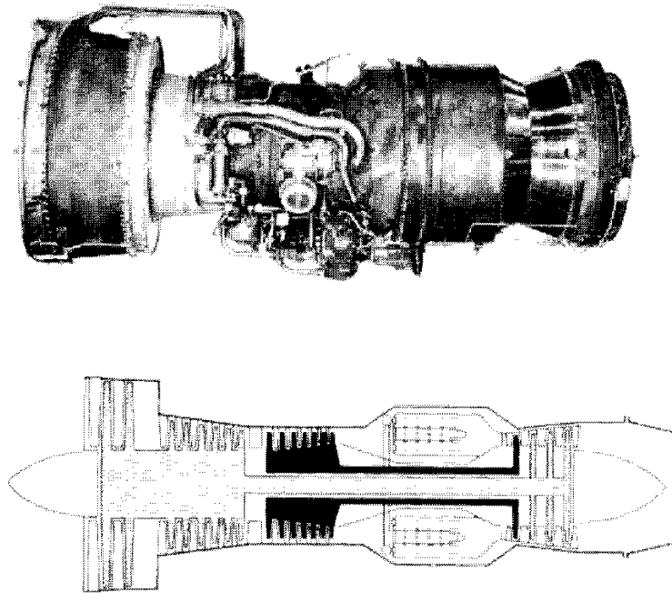
Figure 3.4-5 Turbofan
