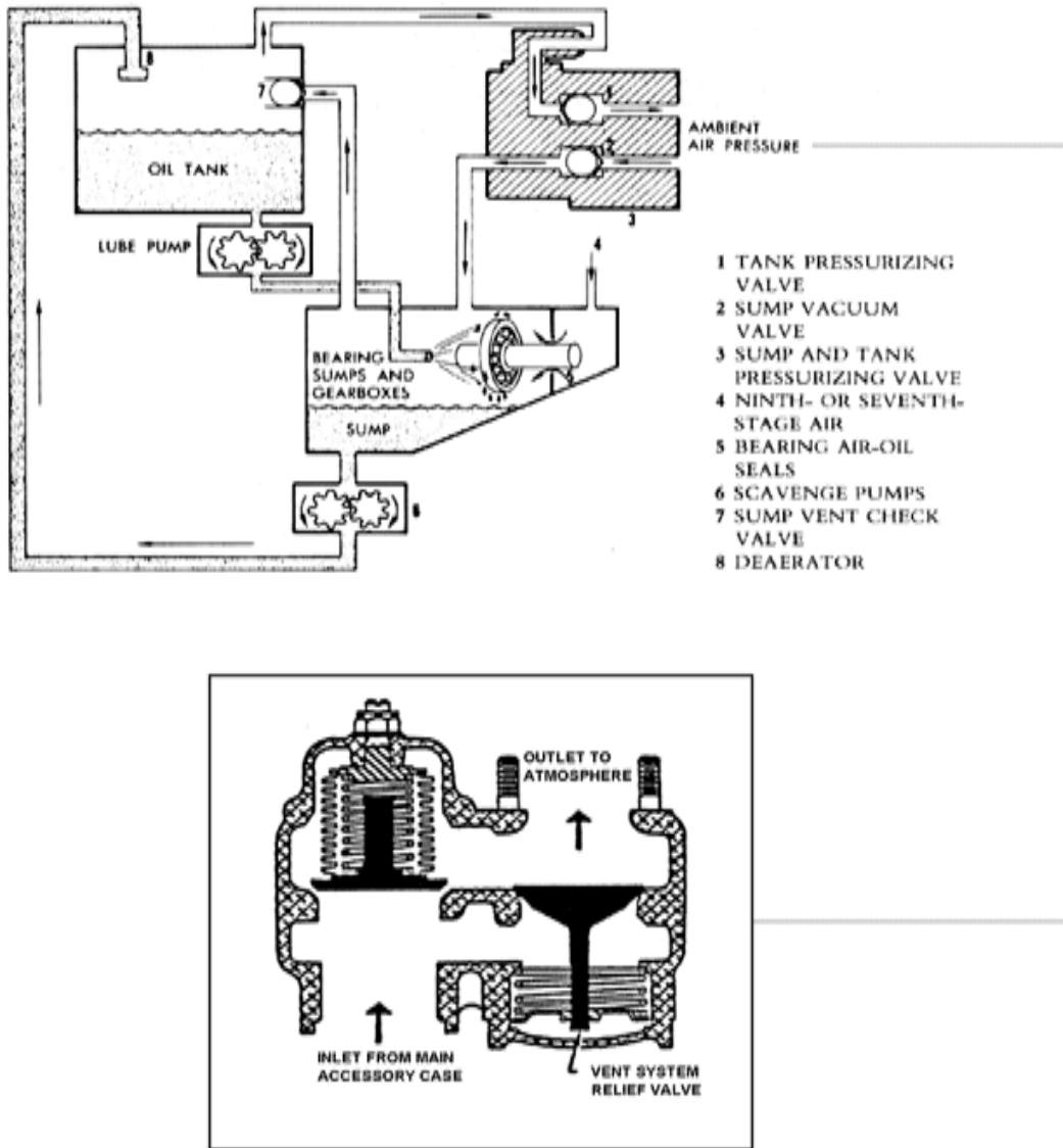
Figure 3.9-7 Breather Pressurizing Valve
