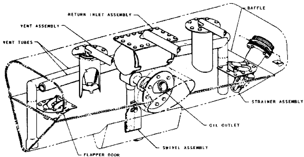
Figure 3.9-3 Swivel Assembly
