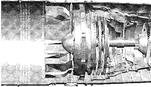
Figure 3.2-19 Turbine Section
