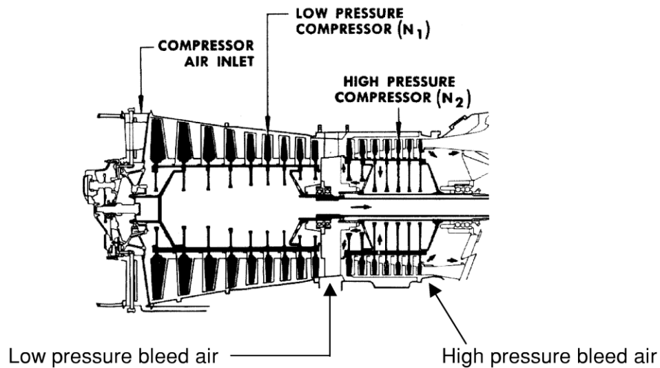
Figure 3.10-2 Low and High Pressure Bleed Air Locations
