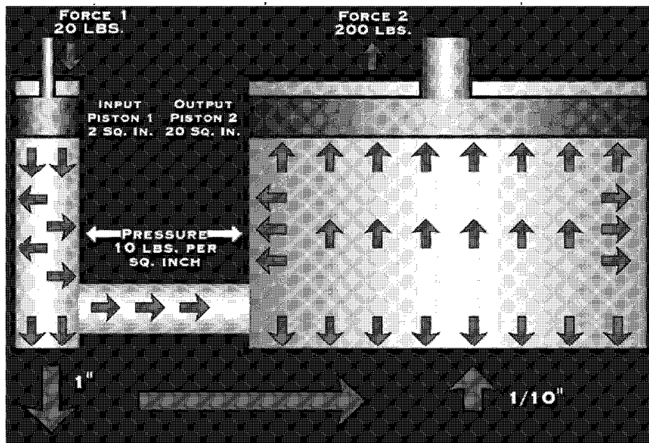
Figure 3.6-3 Hydraulic Example
