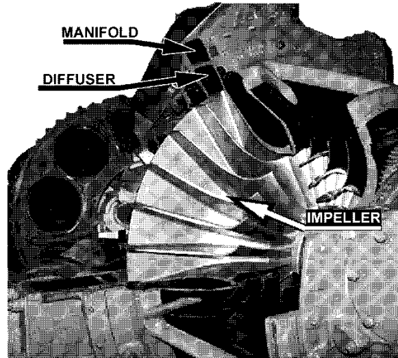
Figure 3.2-8 Centrifugal Compressor
