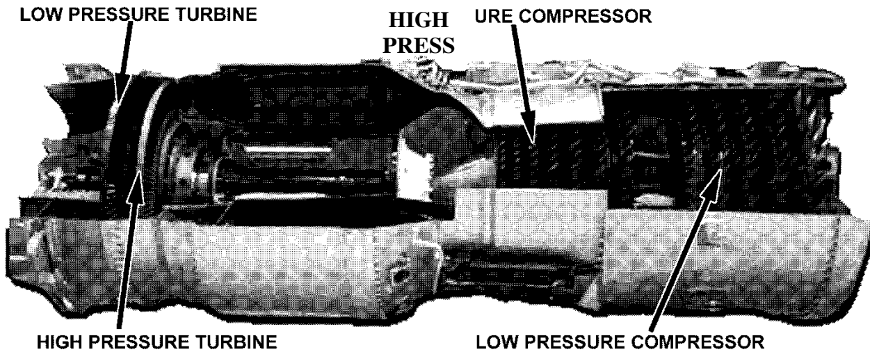
Figure 3.2-21 Dual Turbine
