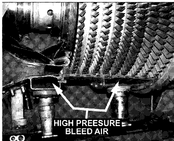
Figure 3.10-1 Bleed Air
