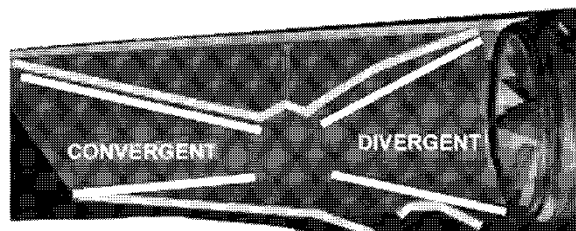
Figure 3.2-6 Supersonic Inlet
