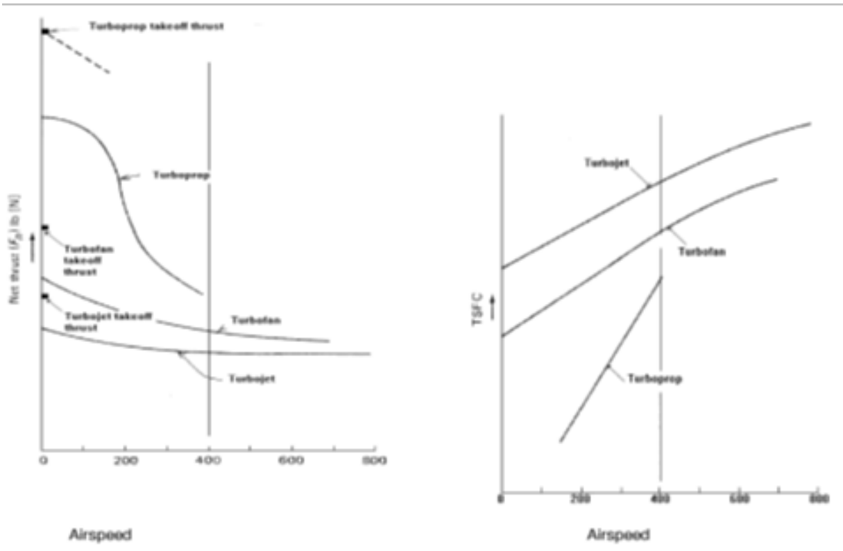
Figure 3.5-7 Thrust Comparison Graph
