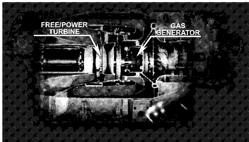
Figure 3.5-9 Turboshaft Engine
