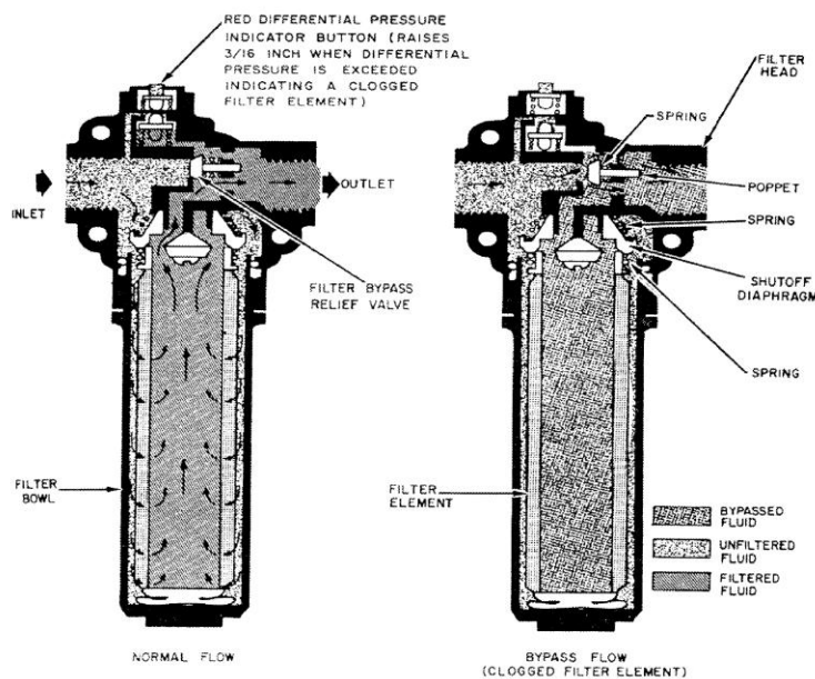
Figure 3.6-9 Hydraulic Filter
