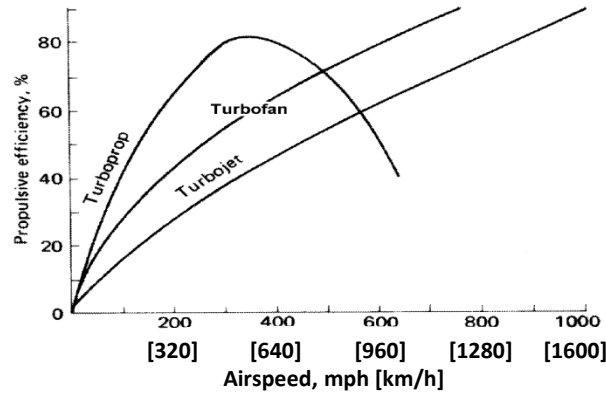
Figure 3.4-2 Engine Efficiency
